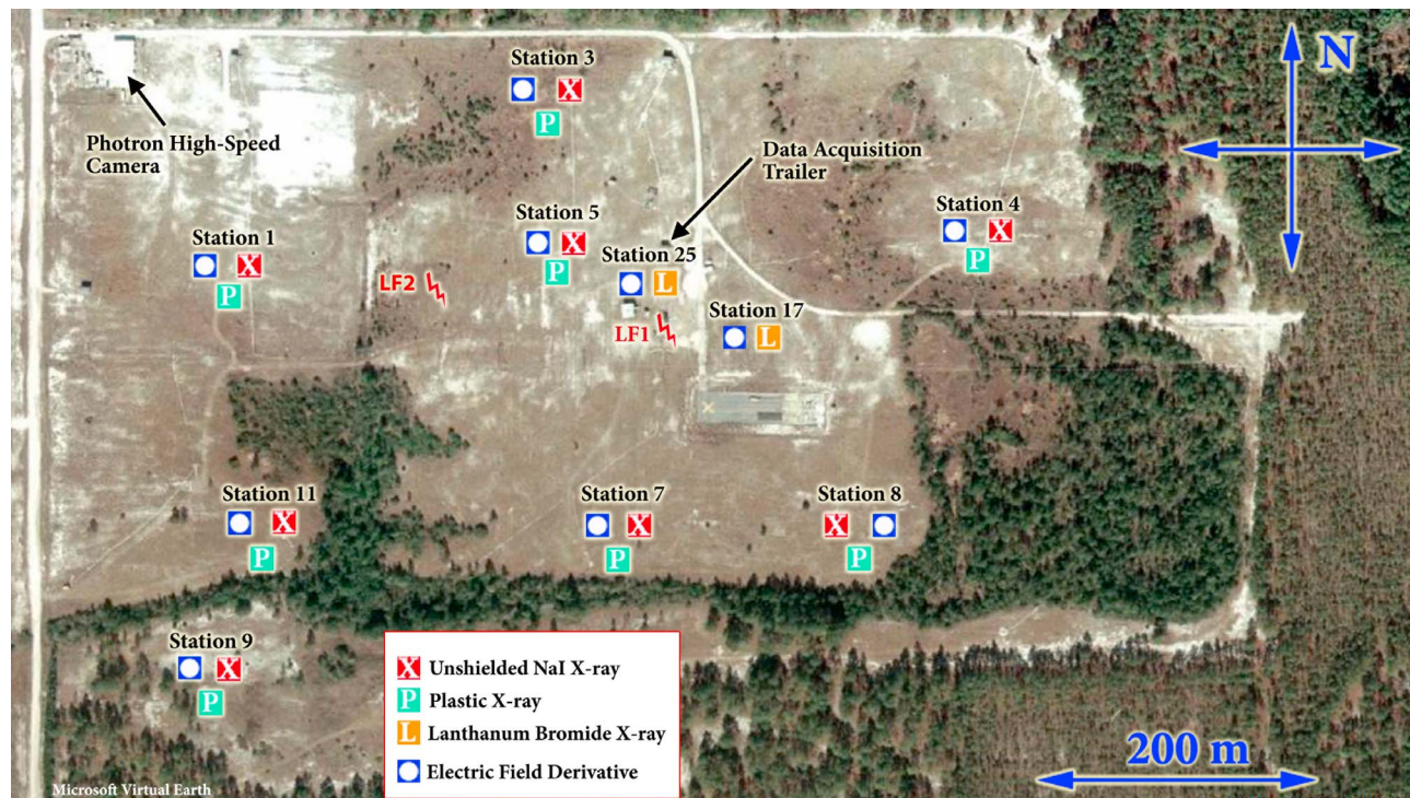
Figure 1. Satellite image of the ICLRT showing LF1 and LF2, the data acquisition trailer, dE/dt and energetic radiation sensor locations, and the Photron high-speed camera location.
