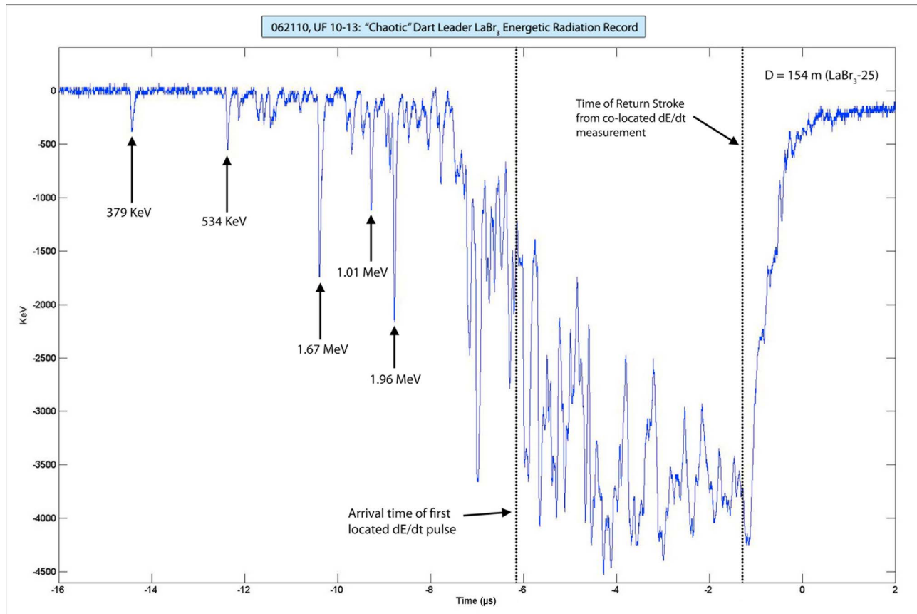
Figure 9. LaBr 3 energetic radiation record for the “chaotic” dart leader on 21 June 2010 measured a distance of 154 m from the lightning channel base. The time of the return stroke and the arrival time of the first located dE/dt pulse are marked by dotted vertical lines. Five detected single photon events are labeled with their respective energies.
