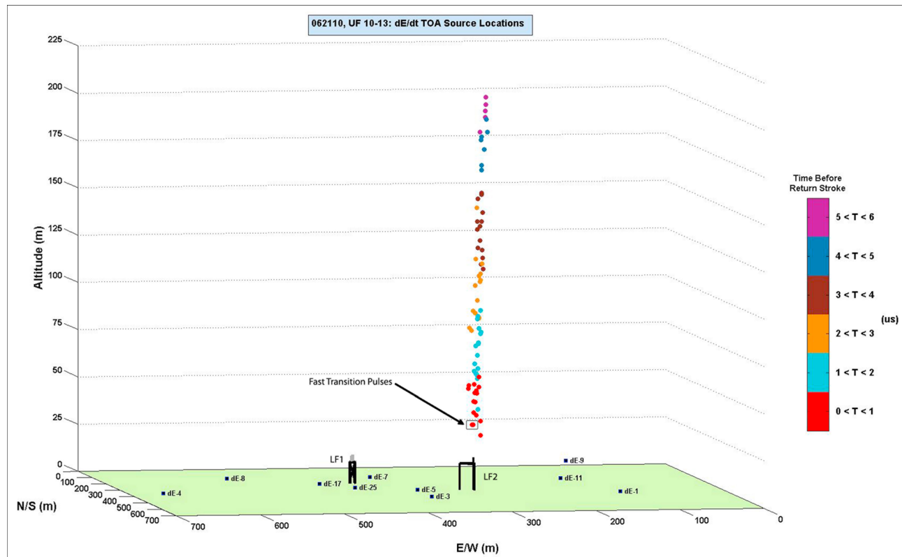
Figure 6. TOA source locations for 75 pulses located during the “chaotic” dart leader on 21 June 2010. Points are color-coded based on calculated emission time relative to the return stroke. The locations of the 10 dE/dt sensors are shown.
